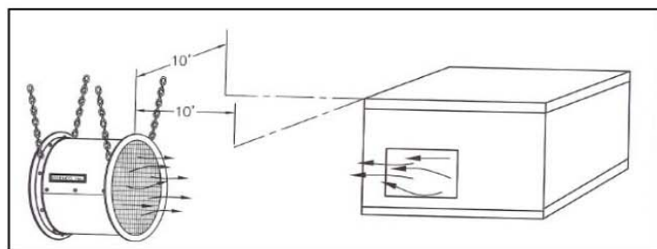
Non-Vented Space Heater
