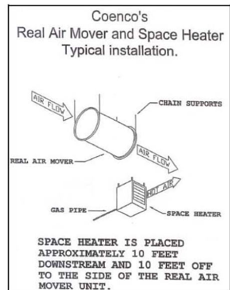
Vented Space Heater
